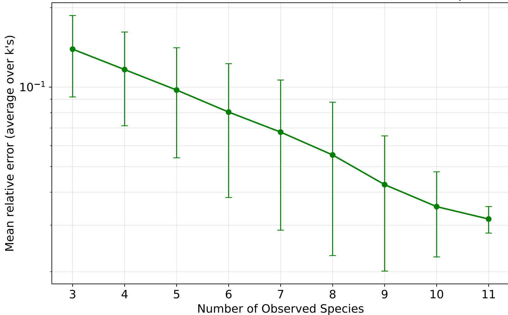
30, 30, 30 — Mean relative error vs number of observed species
